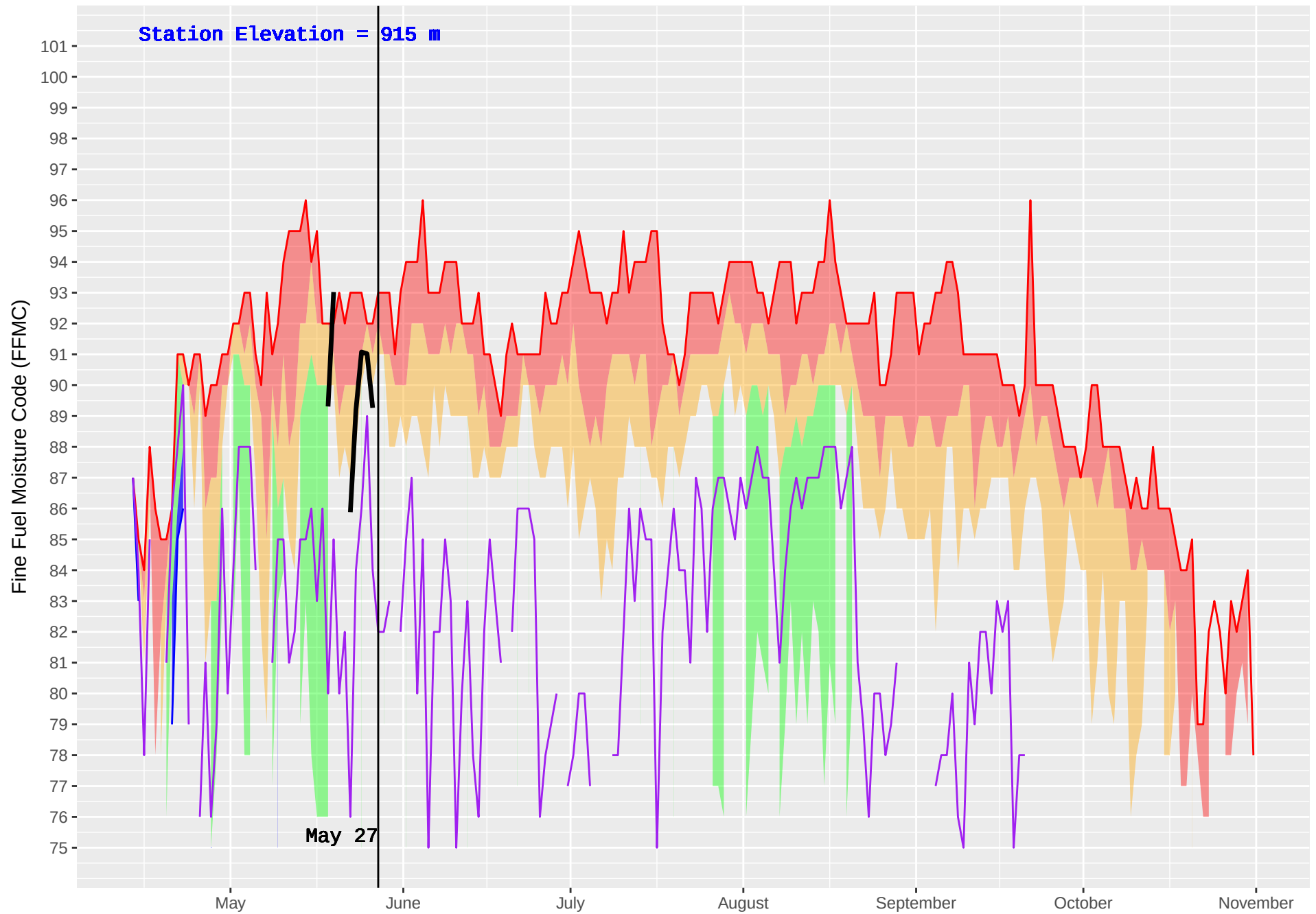
MCLEOD LAKE (153) : Historical (1990–2016) and Current (2018) Noon Fine Fuel Moisture Code (FFMC)
