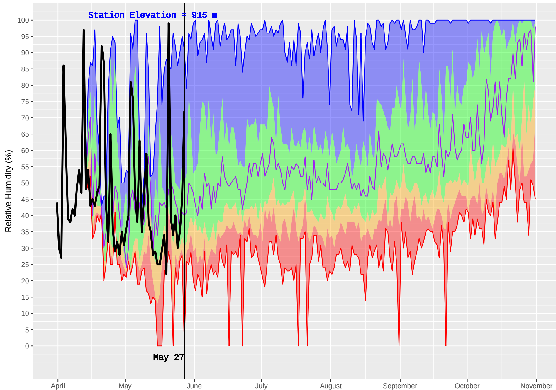
MCLEOD LAKE (153) : Historical (1990–2016) and Current (2018) Noon Relative Humidity
