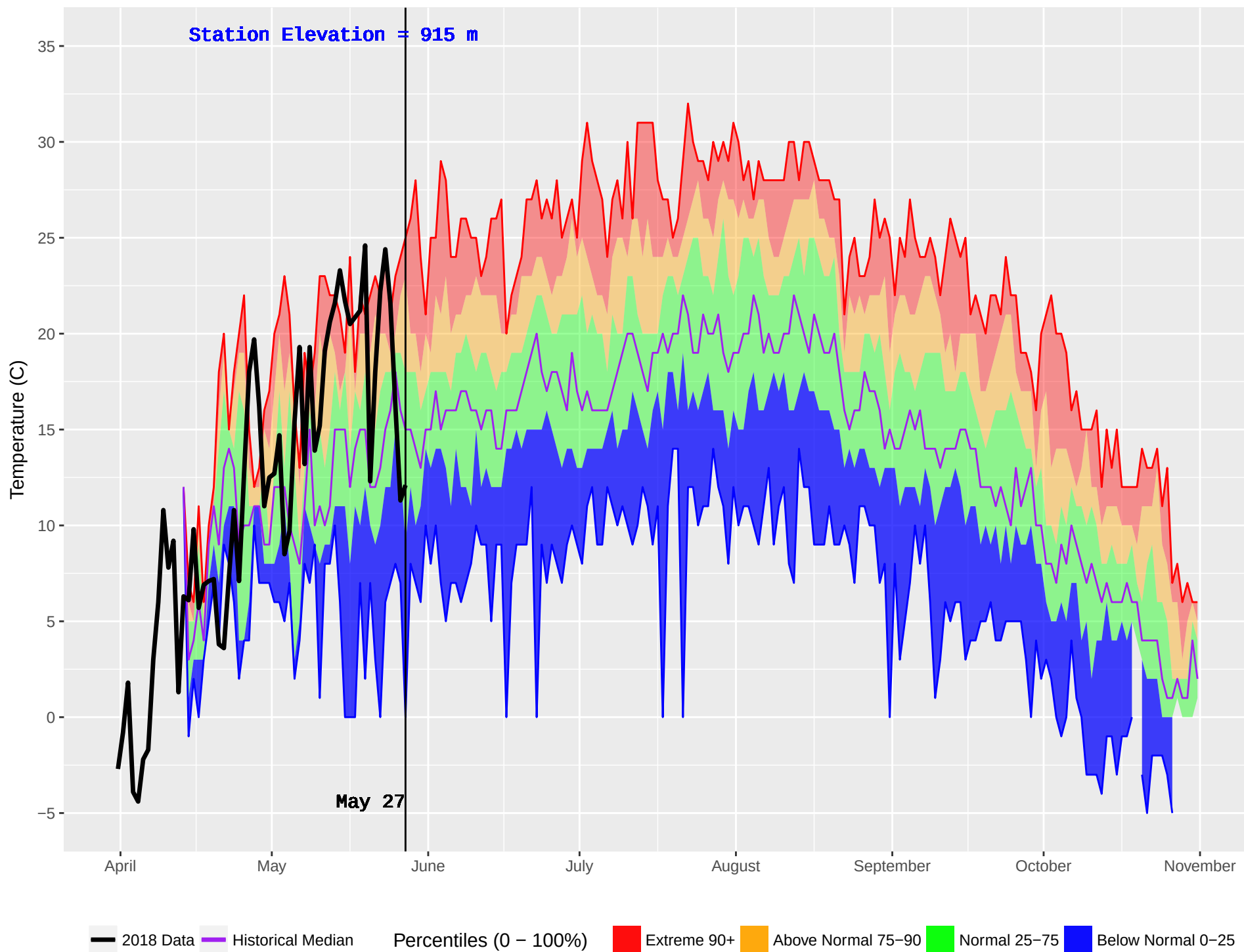
MCLEOD LAKE (153) : Historical (1990–2016) and Current (2018) Noon Temperature
