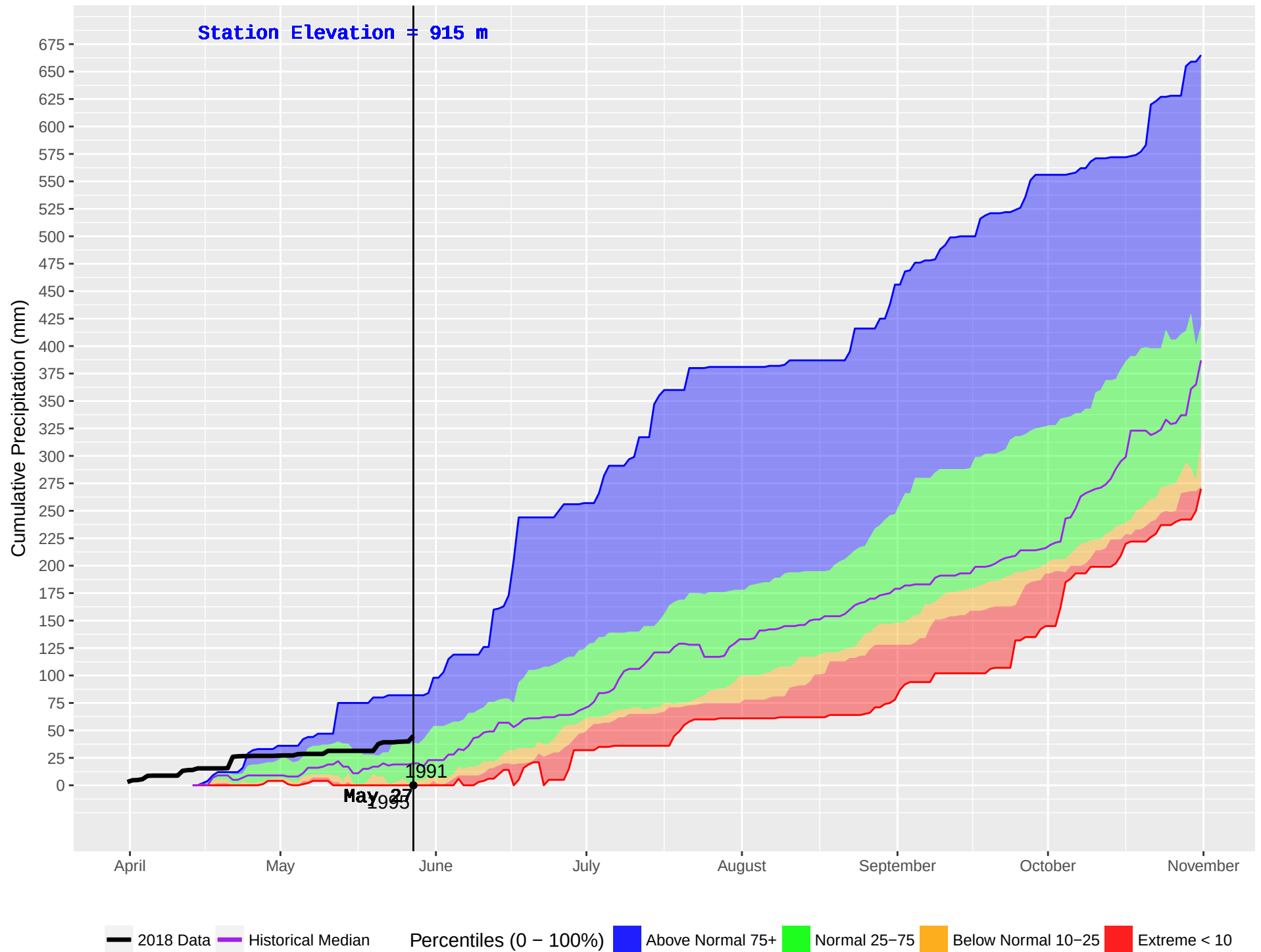
MCLEOD LAKE (153) : Historical (1990–2016) and Current (2018) Noon Cumulative Precipitation
