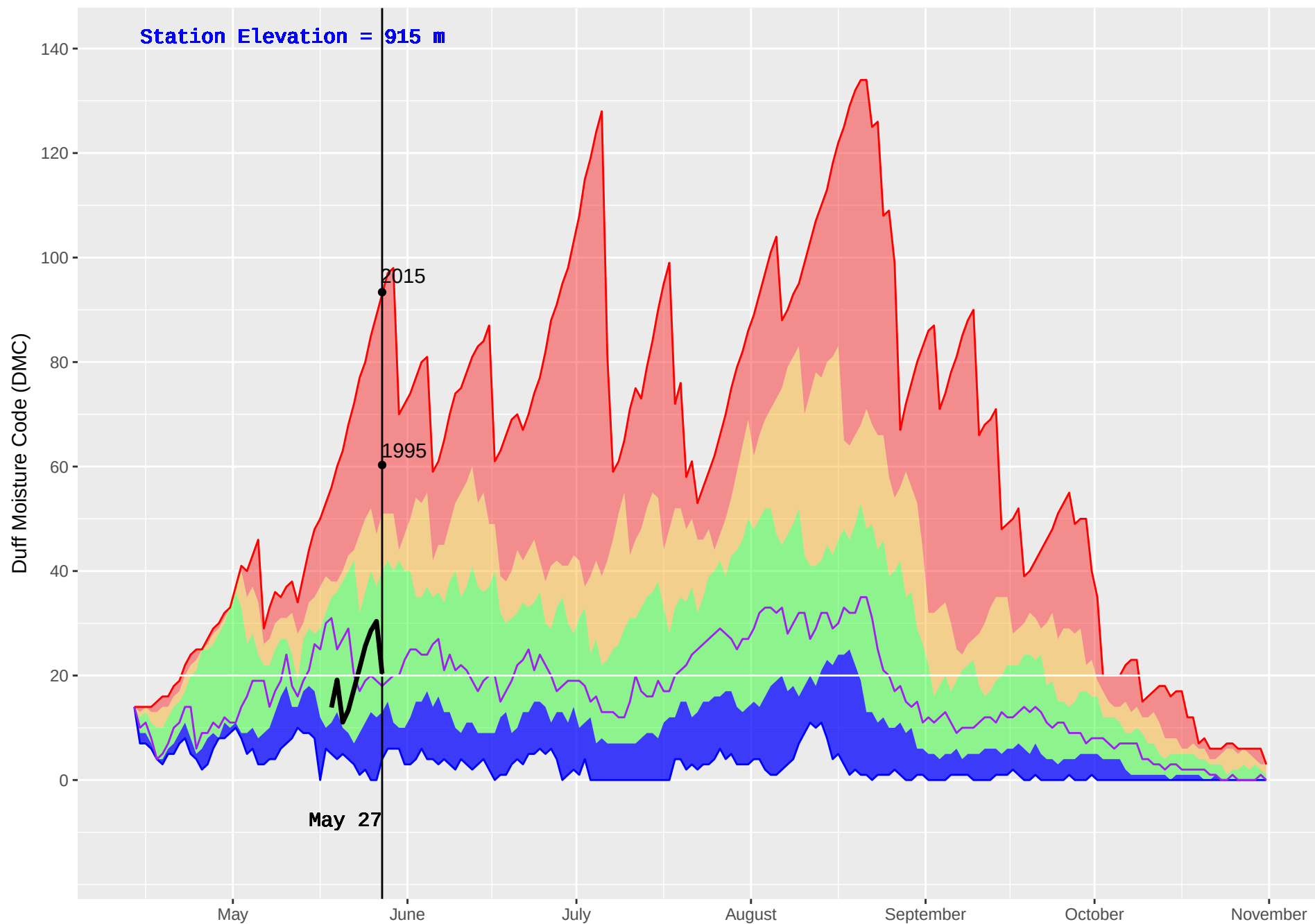
MCLEOD LAKE (153) : Historical (1990–2016) and Current (2018) Noon Duff Moisture Code (DMC)
