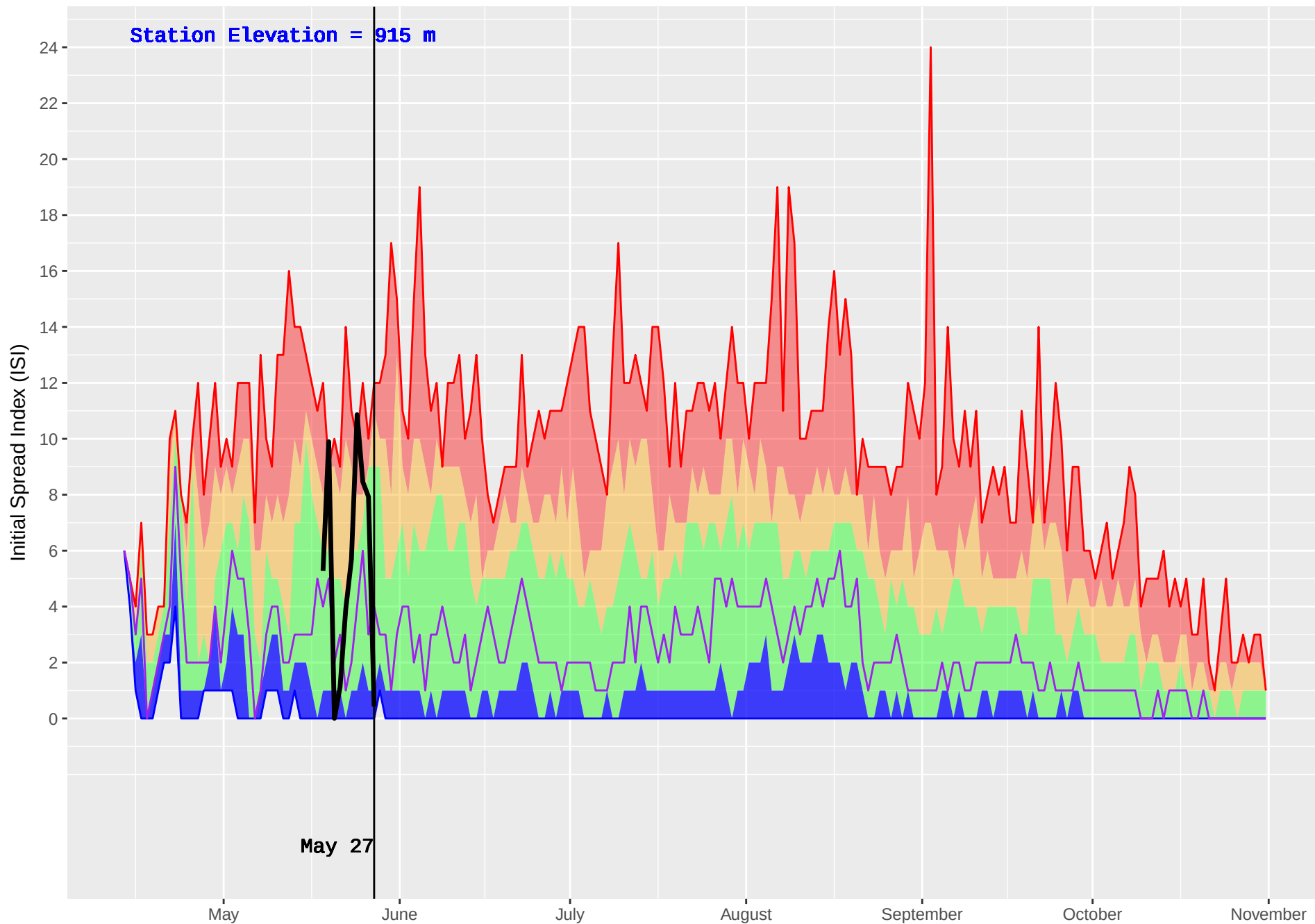
MCLEOD LAKE (153) : Historical (1990–2016) and Current (2018) Noon Initial Spread Index (ISI)
