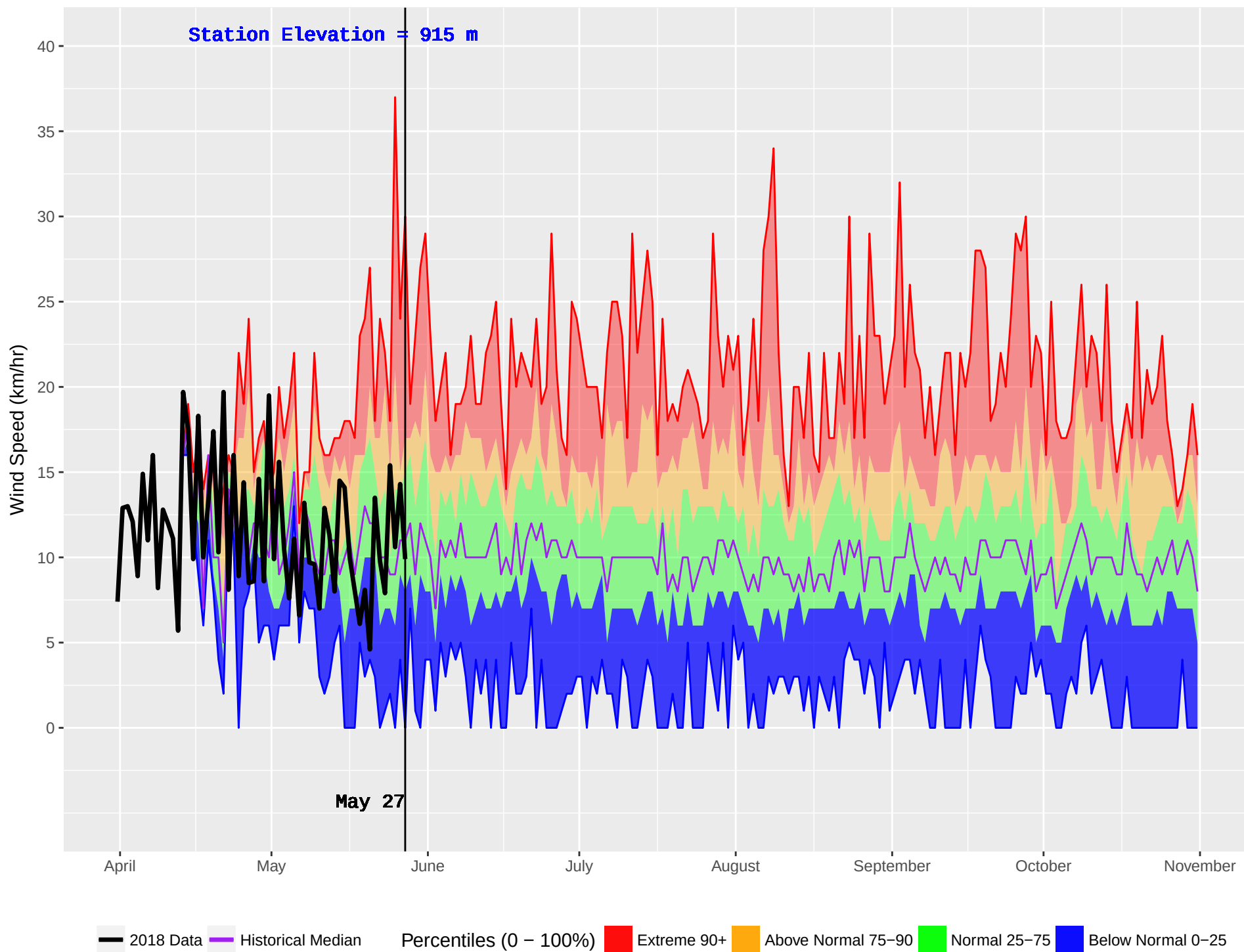
MCLEOD LAKE (153) : Historical (1990–2016) and Current (2018) Noon Wind Speed
