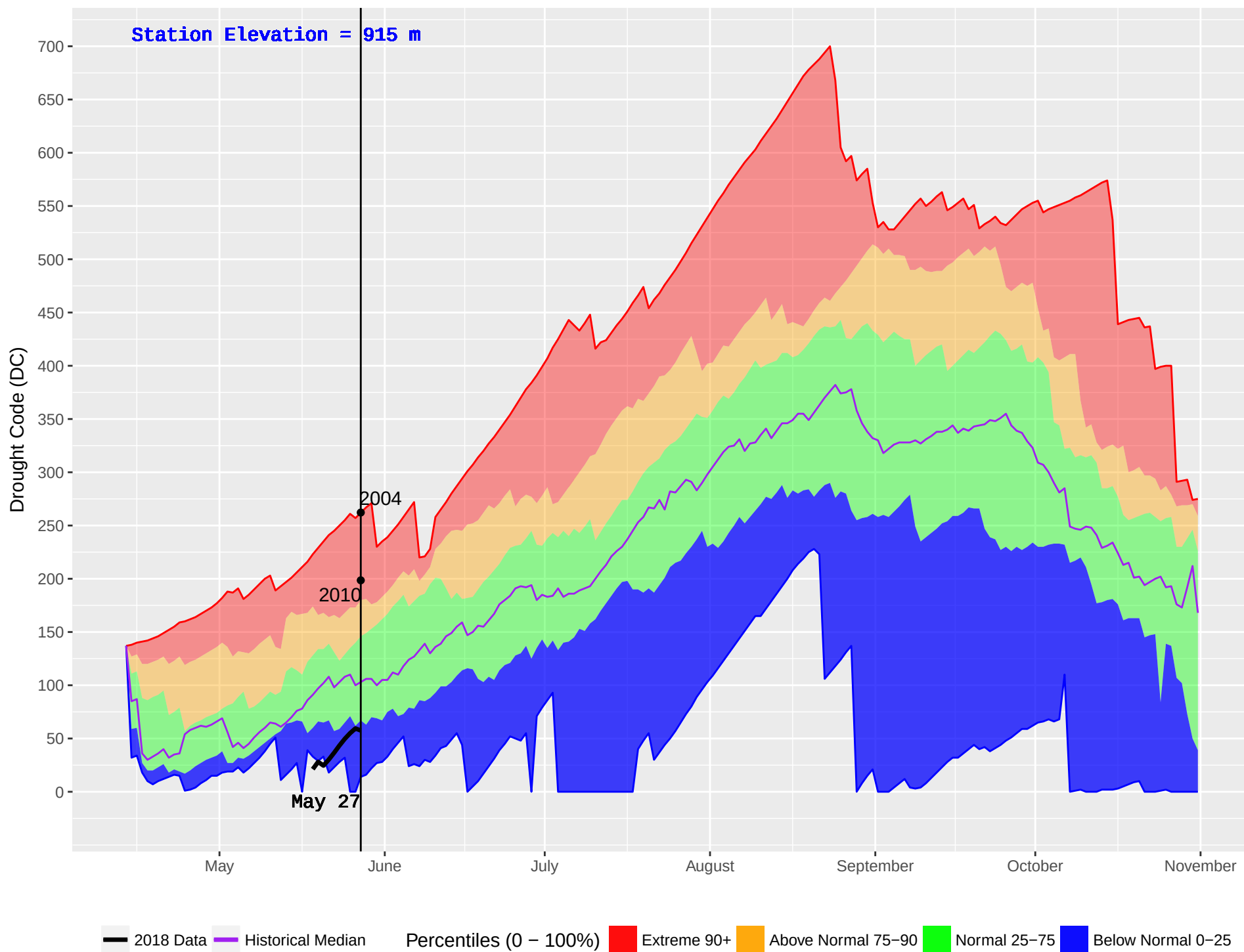
MCLEOD LAKE (153) : Historical (1990–2016) and Current (2018) Noon Drought Code (DC)
