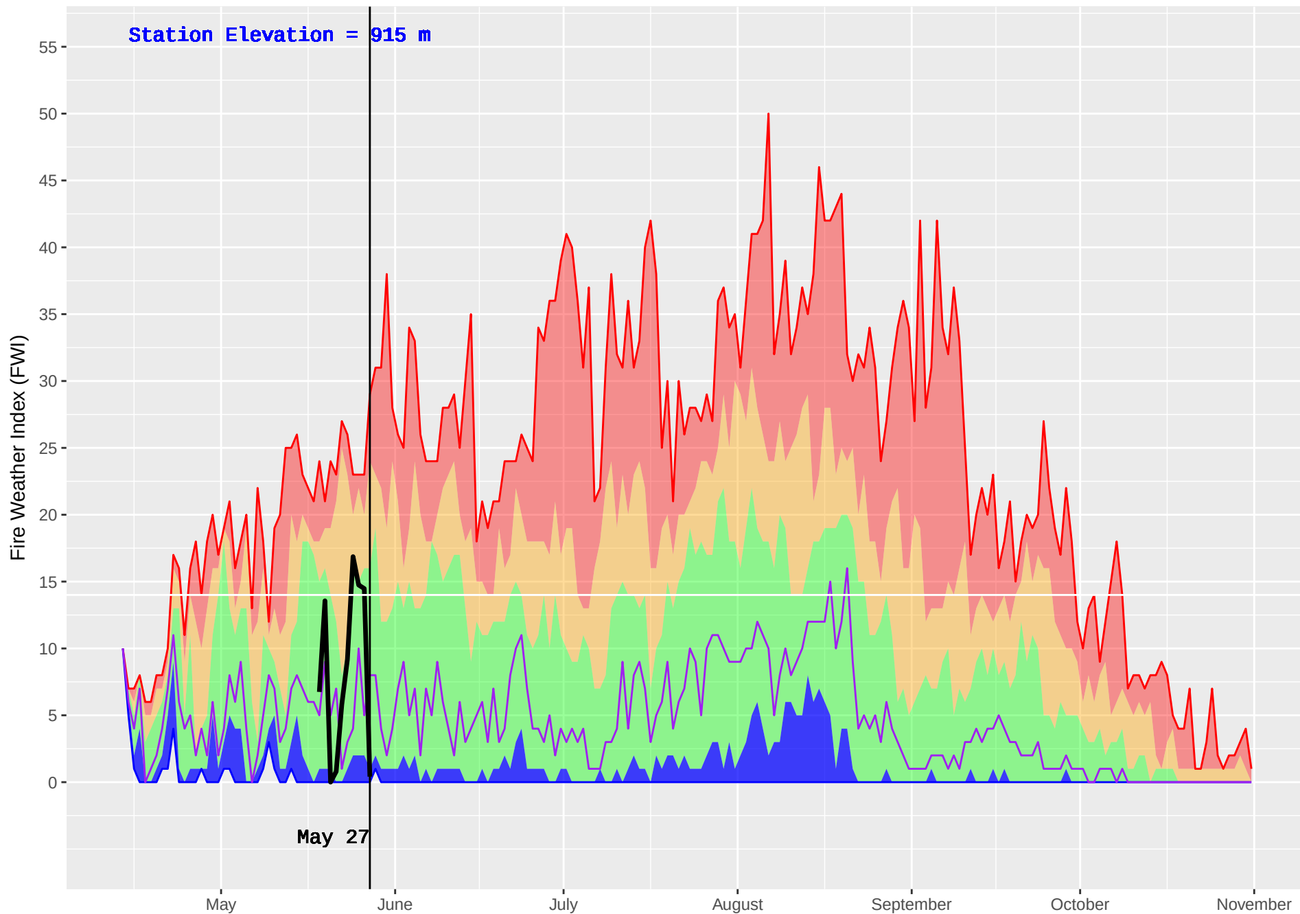
MCLEOD LAKE (153) : Historical (1990–2016) and Current (2018) Noon Fire Weather Index (FWI)
