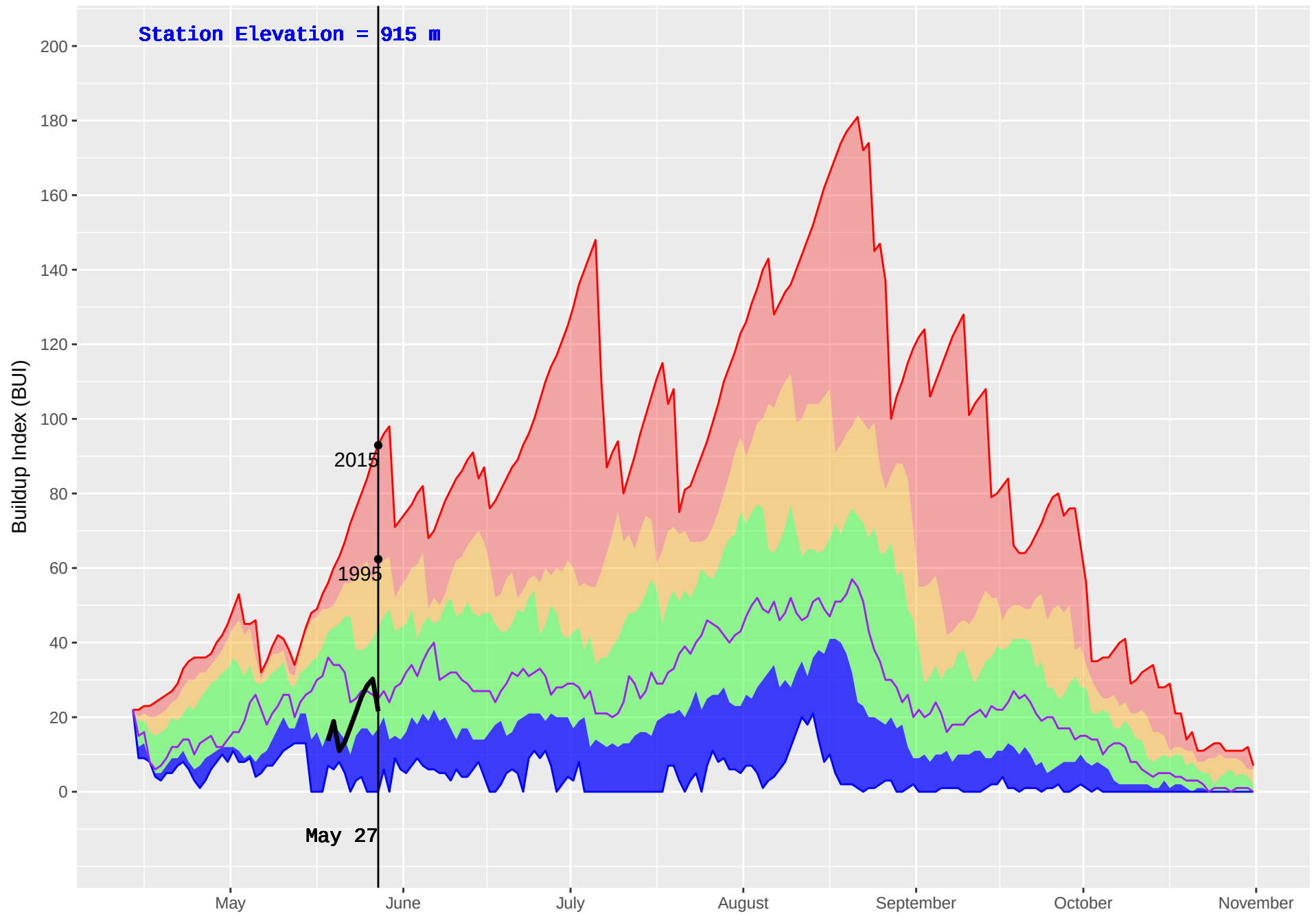
MCLEOD LAKE (153) : Historical (1990–2016) and Current (2018) Noon Buildup Index (BUI)
